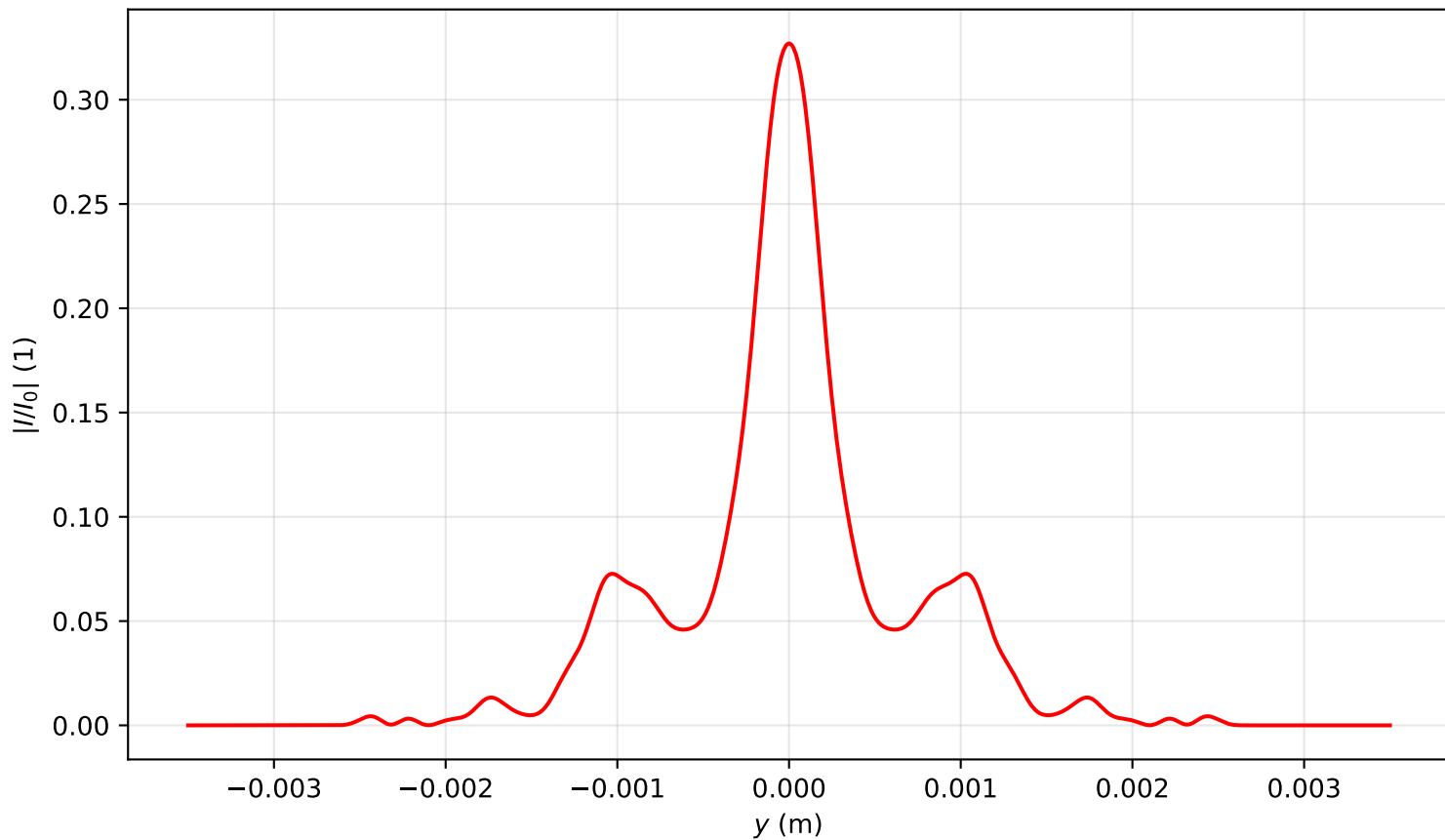
Intensity profile I(x = 0, y, z = 2.627)/I_0 , P_{in}=5.5P_{cr} , artificial time
